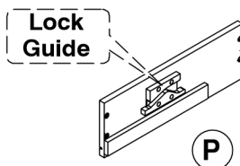
P LEFT Drawer Side (Right Hand) x 3
