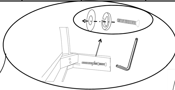
front leg*2PCS
